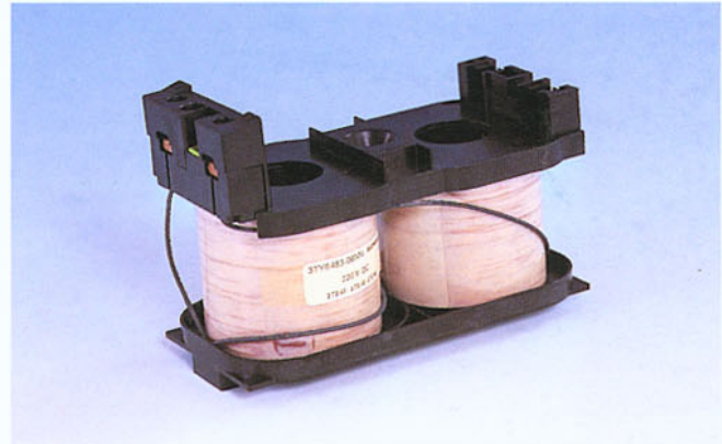
3TC48 Contactor coil
